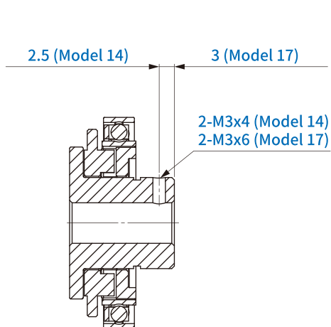
Wave generator hub shape for models 14 and 17 (no keyway)
